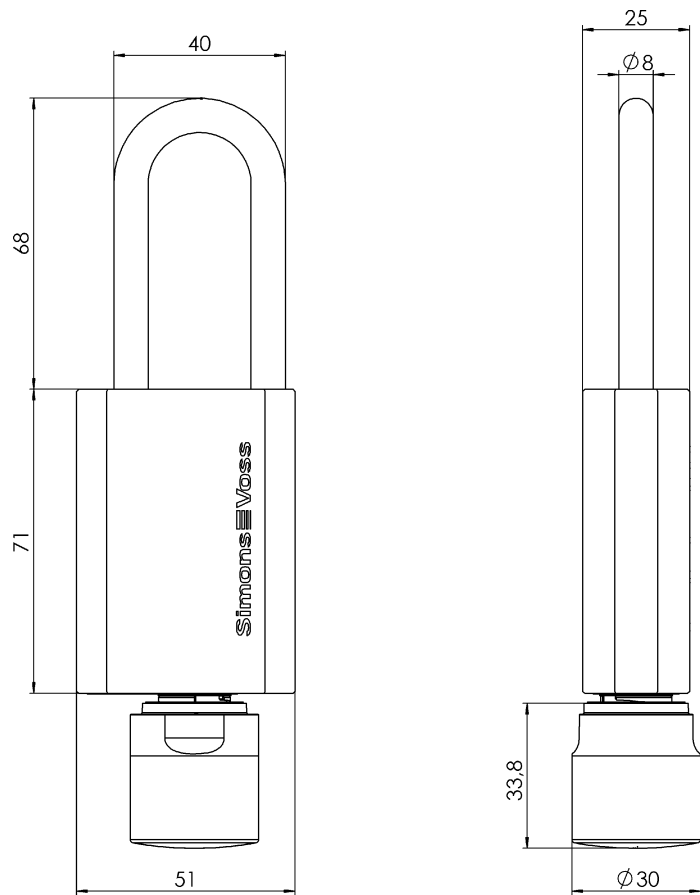
Padlock 8 mm - Active (PL)
